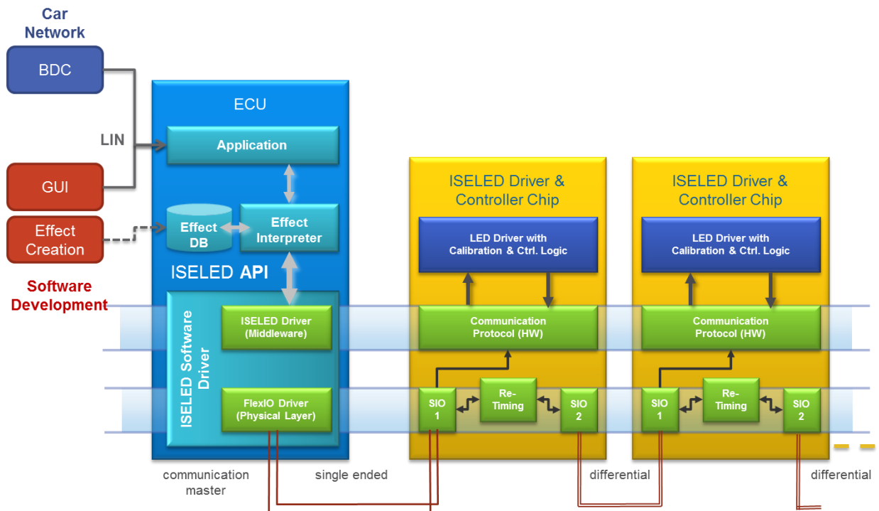
ISELED software architecture
